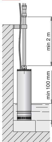
3.93.00770 Construction without float switch
