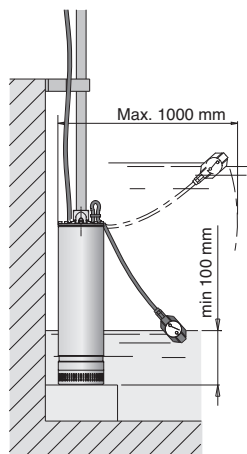
3.93.00772 Construction with float switch
